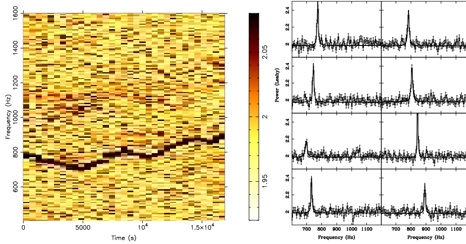
Figure 1. Left Panel: Dynamic power spectrum of the source 4U 1728–34. Right Panel: Power spectra of some selected intervals.
